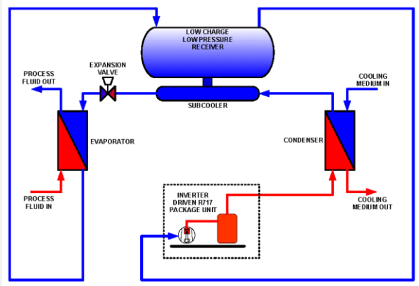
Simplified Refrigeration System Drawing
